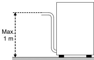
Free drain
