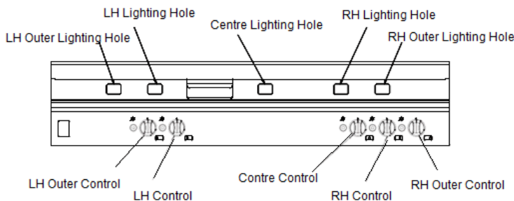
Figure 7 - G31525 Panel Layout
