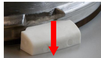
6. Continue to rotate the dust guard until the white guide block aligns with the cut out in the drip cup ridge.
