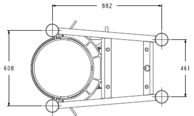
FIGURE 2. H600S STANDARD PLANETARY FOOD MIXER OVERALL DIMENSIONS (HUB ATTACHMENT OPTIONAL).
