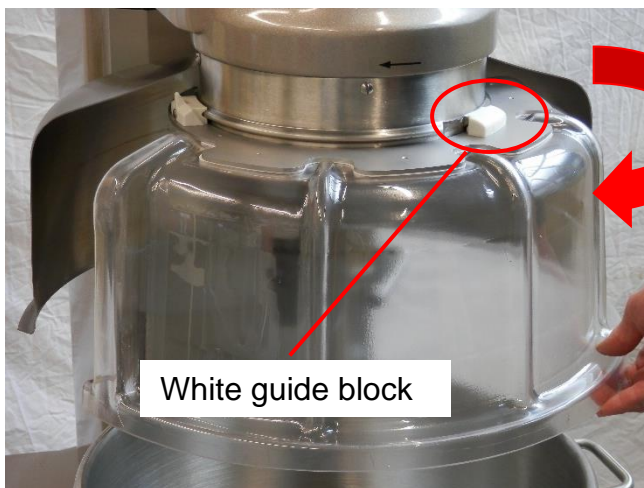
6. Continue to rotate the dust guard until the white guide block aligns with the cut out in the drip cup ridge.
