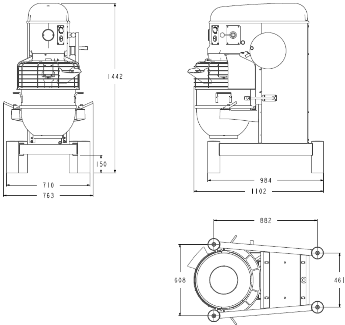
FIGURE 5. H800S MARINE PLANETARY FOOD MIXER MODEL OVERALL DIMENSIONS (HUB ATTACHMENT OPTIONAL).
