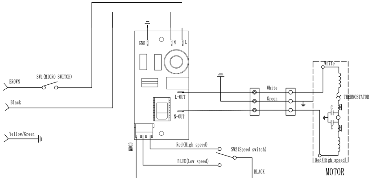
DM1264(HMD300-CE) Schematic electrical diagram
