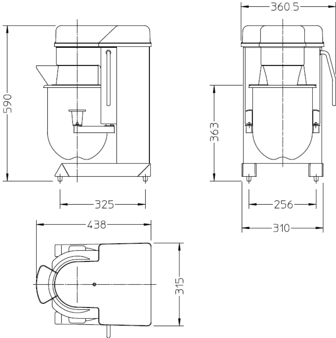
FIGURE 2. HSM10N PLANETARY FOOD MIXER OVERALL DIMENSIONS
