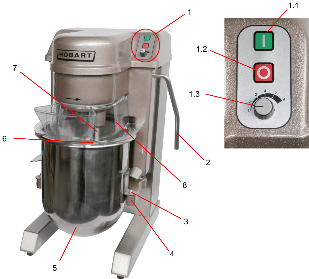
FIGURE 1. MIXER COMPONENT IDENTIFICATION.
