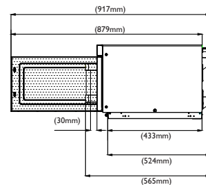
SIDE VIEW (DOOR OPEN)
